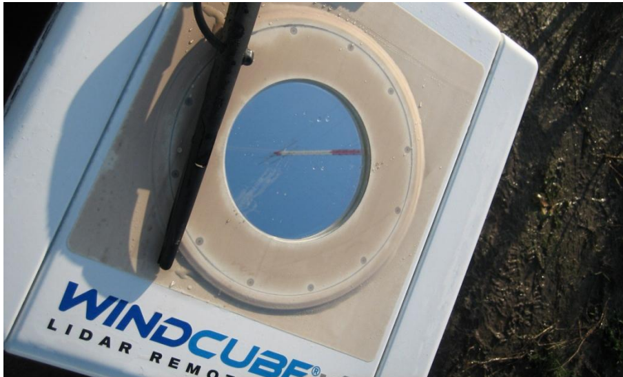
LIDAR can complement a met mast campaign, allowing for a shorter mast with better understanding of extrapolation to hub height [Project reference: Delfzijl Noord, 2011]
