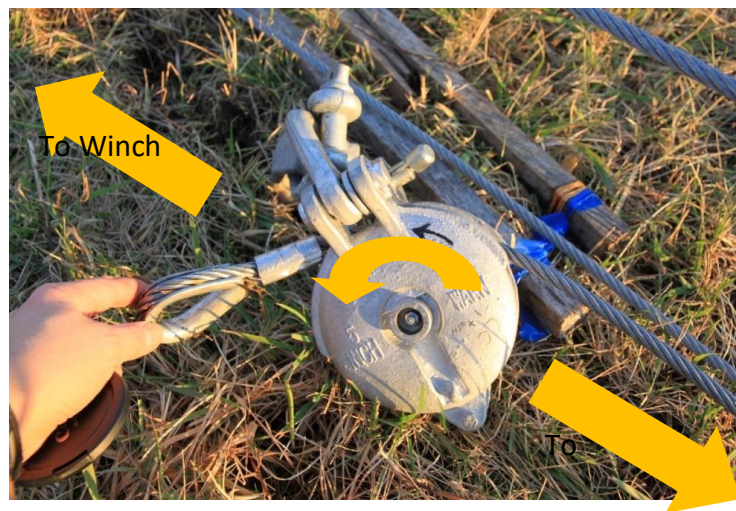
Picture 3-78: Reeving through pulley #5
