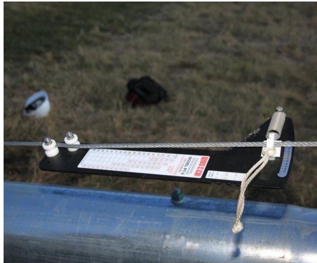
Picture 3- 81: Correct use of tension gauge
