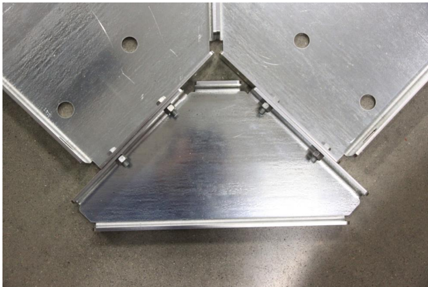
Picture 3-3: Baseplate Assembly
