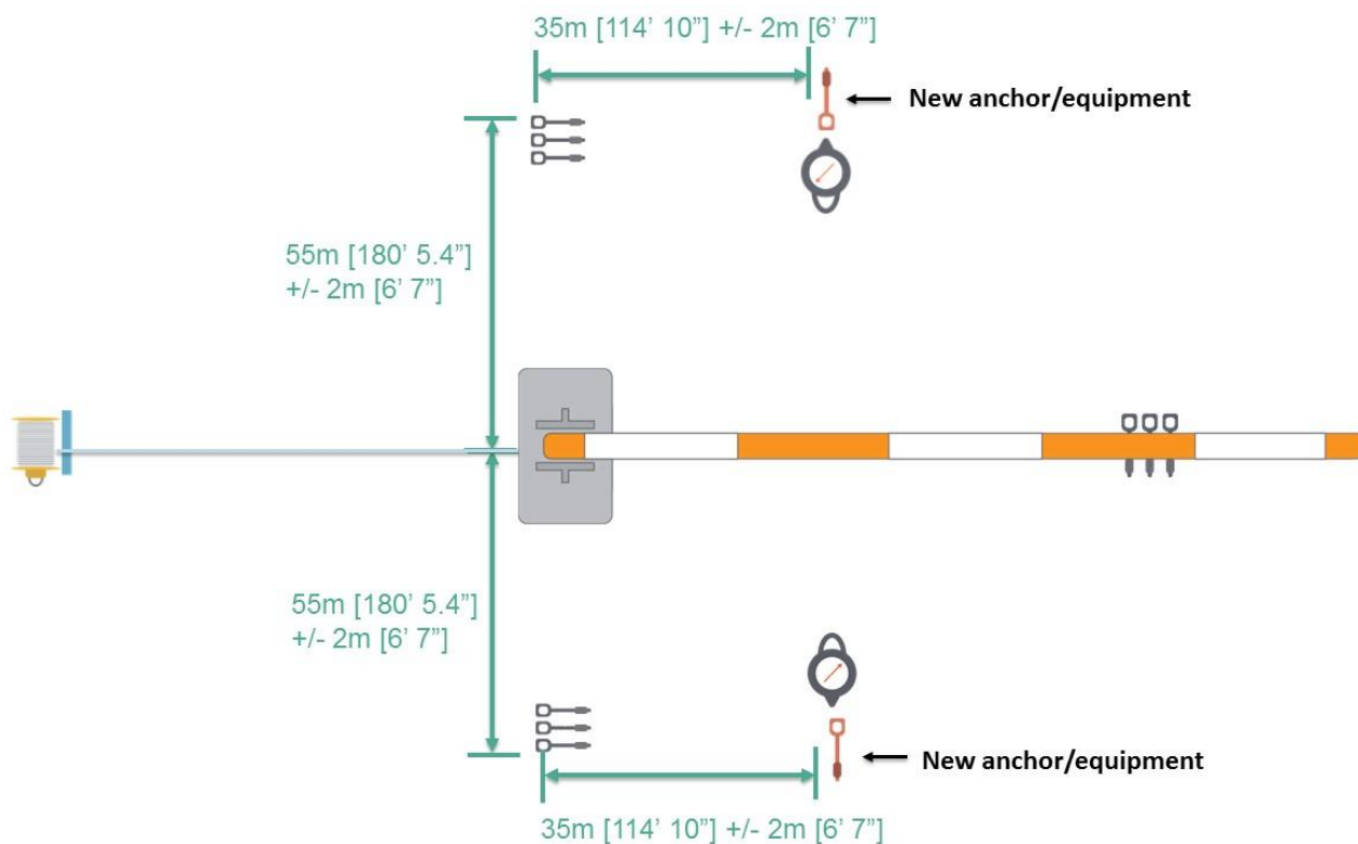
Picture 2-5: Layout drawing showing location of back stay tensioning system
