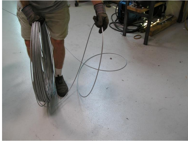
Picture 3-32: Unroll guy wires Incorrect!
