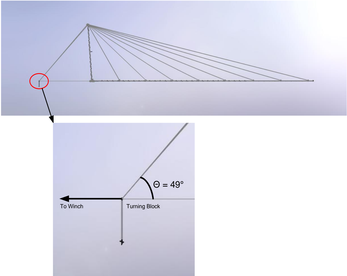
Picture A-3: Angle of winch cable at maximum load
