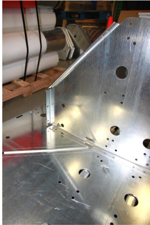
Picture 3-6: Baseplate Assembly
