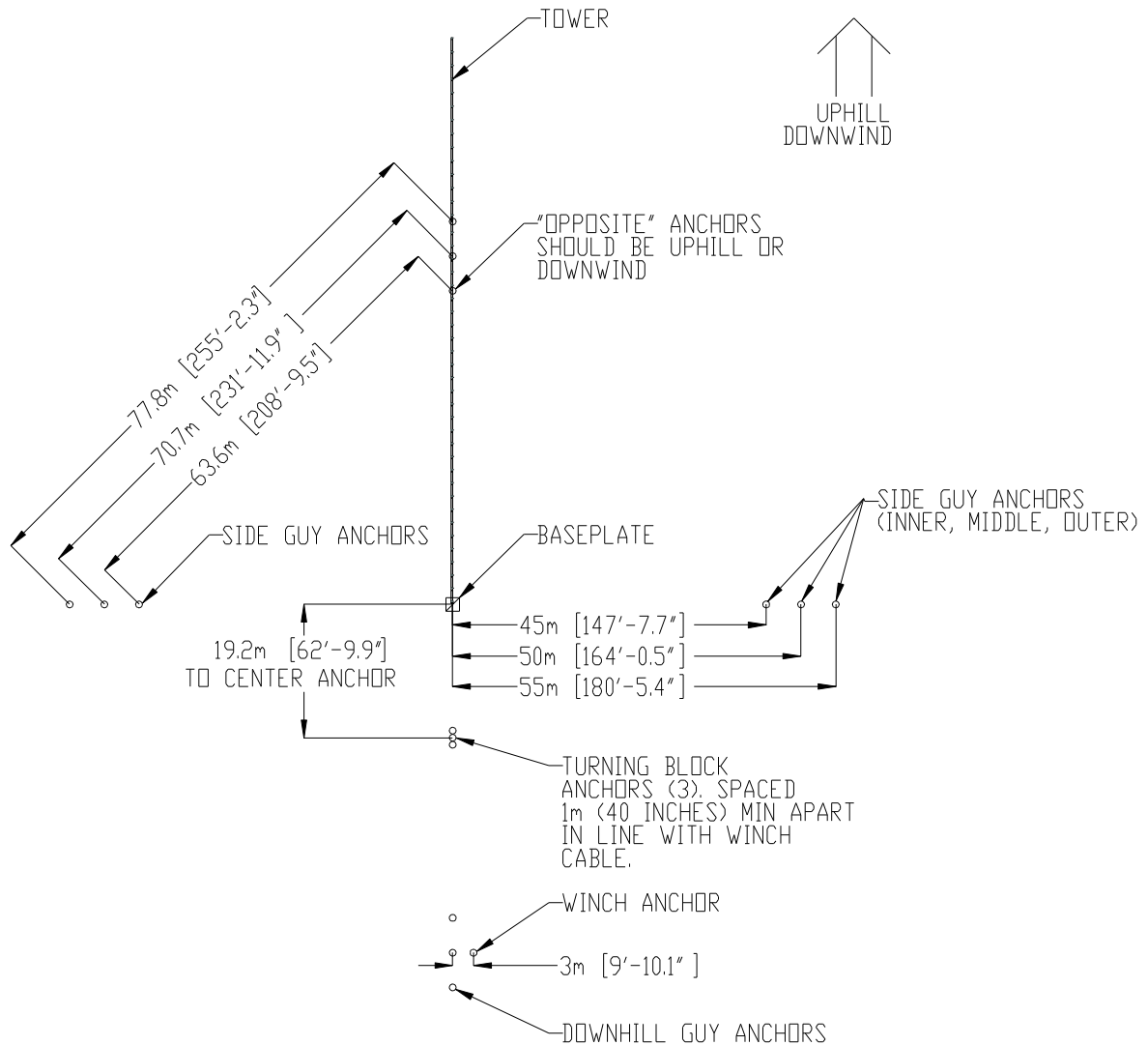
80m XHD TALLTOWER SITE LAYOUT
