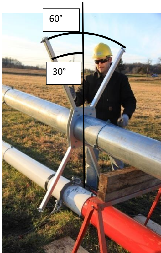
Picture 3-46: Install jumper struts
