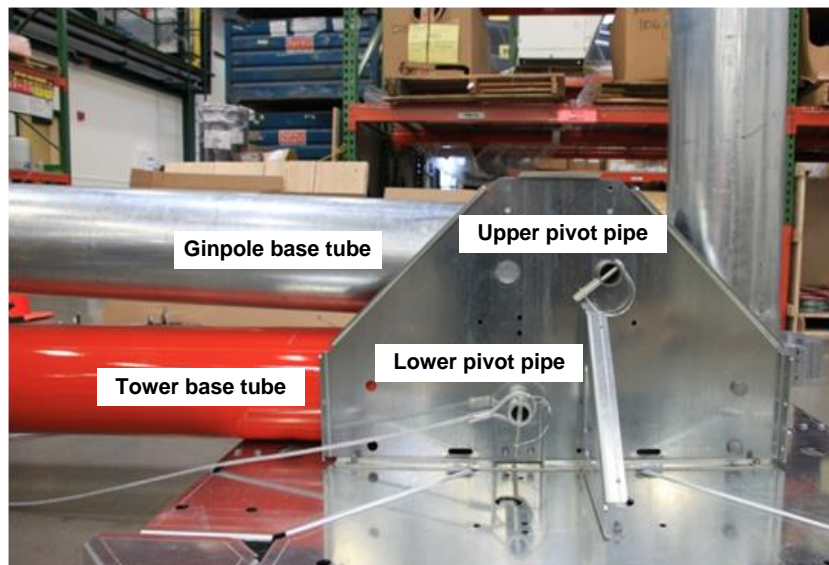
Picture 3-15: Baseplate fully assembled/ready for lifting
