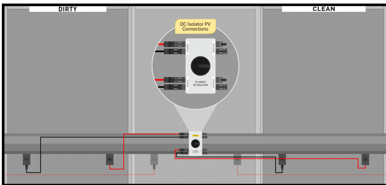
Example DC Isolator Location
