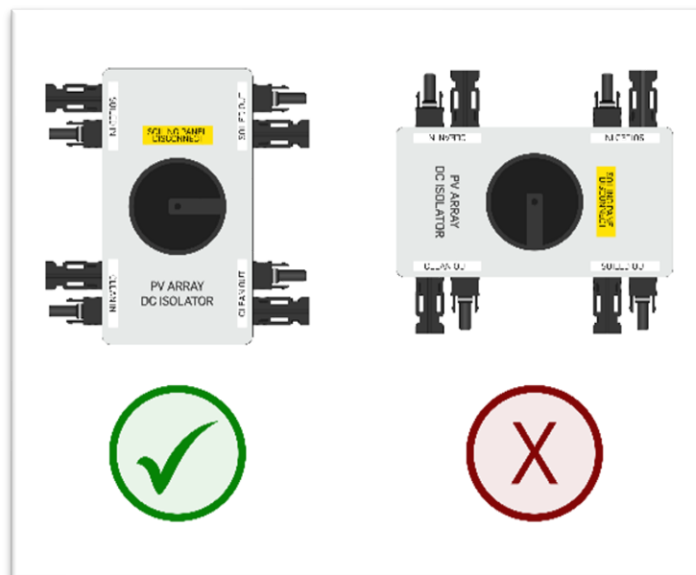
DC Isolator - Acceptable Mounting Orientations
