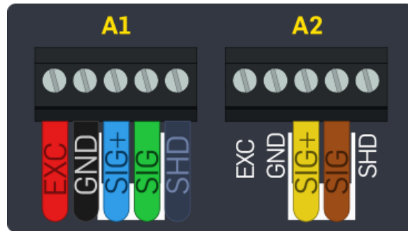
LOGR-S, Analog, Sensor Wiring
