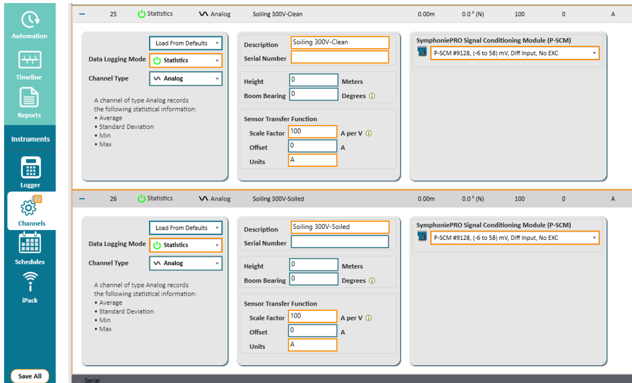
Figure 11: Channel configuration for S.I.M | 300V
