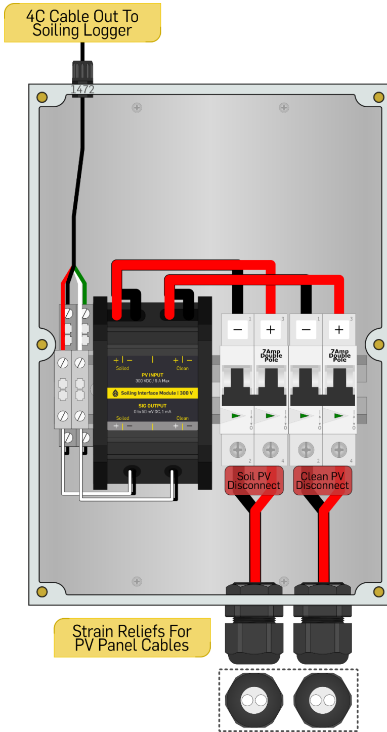
Figure 17: Soiling Interface Module | 300V J-Box
