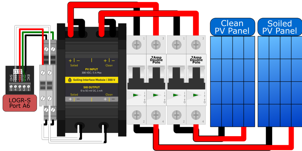
Figure 18: Soiling Interface Module | 300V – Flow Diagram | LOGR-S
