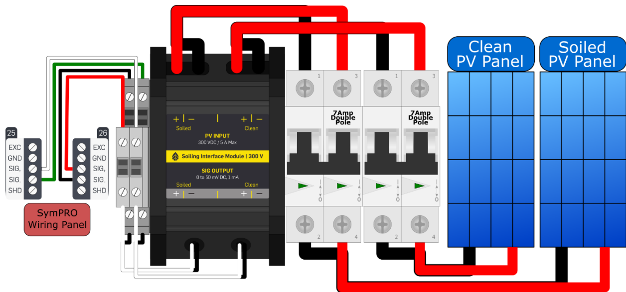
Figure 19: Soiling Interface Module | 300V – Flow Diagram | SymphoniePRO
